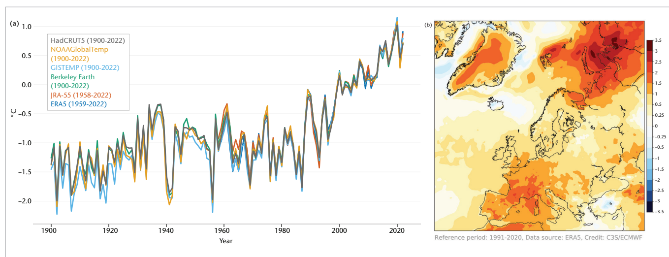
Figure 1. (a) Annual average surface air temperature anomaly (°C) over Europe, as defined by the WMO Region VI (see the Region domain subsection under Data sets and methods), for 1900–2022, using data from six data sets (for land only), and (b) for 2022 from ERA5 reanalysis, compared to the 1991–2020 reference period.
