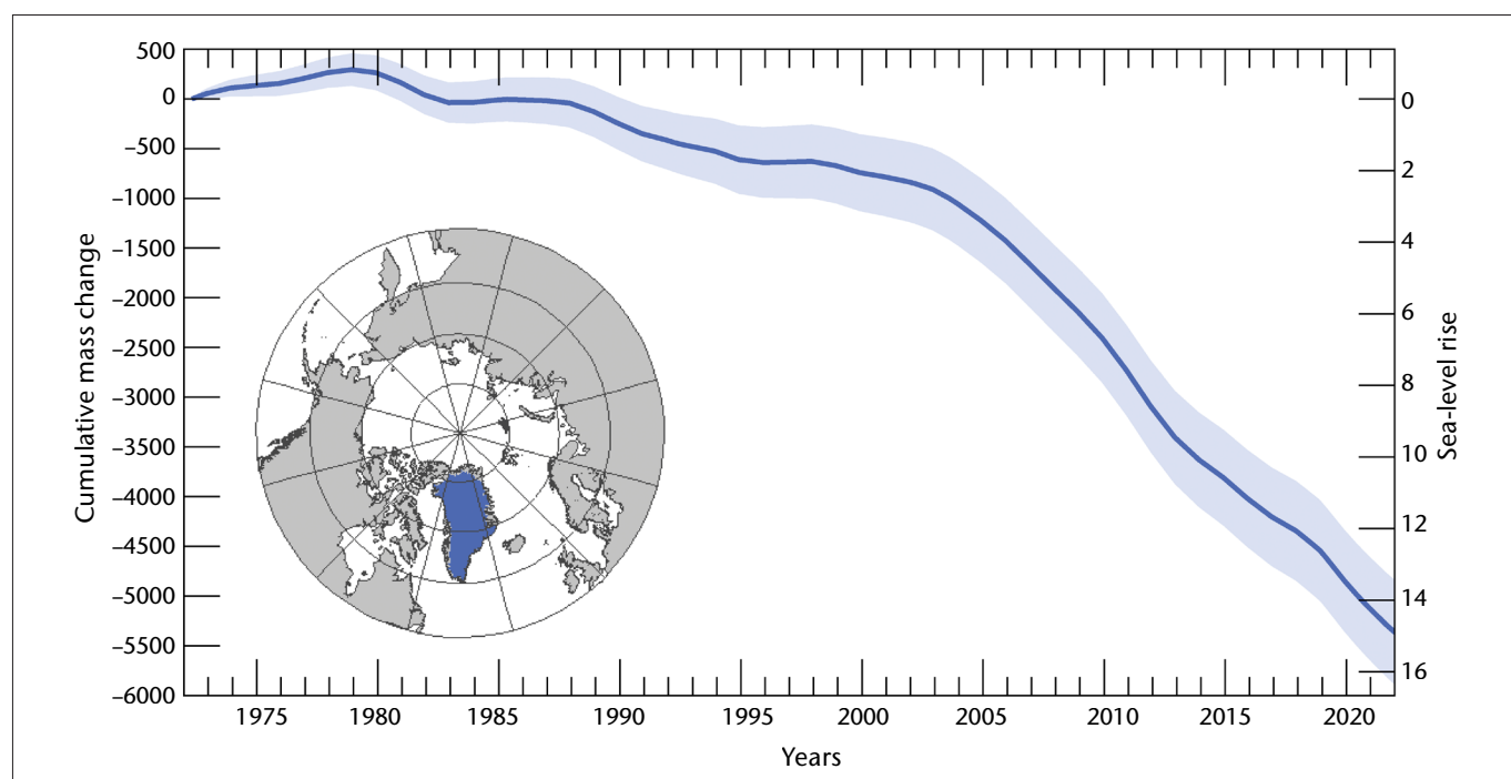
Figure 4. Cumulative mass balance of Greenland Ice Sheet and the corresponding contributions to global mean sea level, between 1972 and 2021 (year label indicates the start of the year). The shading represents the cumulative uncertainty.
