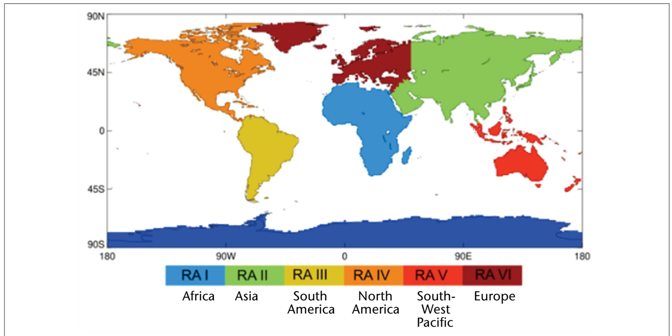
Figure 19. Map of WMO Regional Association (RA) areas. WMO Region VI is the focus of the present report.
