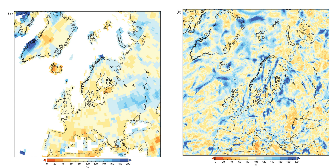
Figure 2. (a) Relative anomaly of the annual precipitation total in 2022 with reference to 1991–2020. Yellow, orange and red colours indicate a precipitation deficit while blue regions experienced a precipitation excess. (b) Deviation of the highest daily precipitation amount (RX1) in 2022 from the reference period 1991–2020. Blue indicates regions where RX1 is higher than the annual mean, while in brownish coloured regions the RX1 was below the long-term mean.
