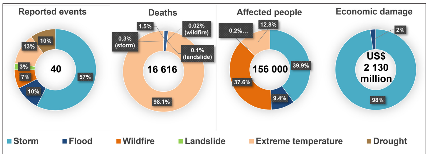
Figure 10. Weather-, climate- and water-related extreme events in Europe during 2022. Note: Impact numbers for some disaster occurrences may be lacking due to data unavailability. Some transnational events may be reported individually by the affected countries.
