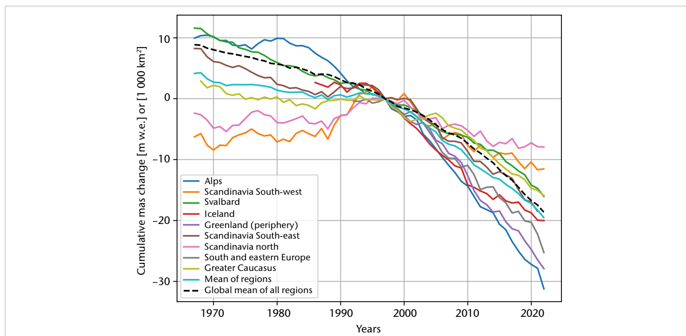
Figure 3. Cumulative glacier mass changes in Europe from 1967 to 2022, for glaciers with long-term records in nine different regions. Mass balance values are given in metres of water equivalent (m w.e.), relative to 1997.
