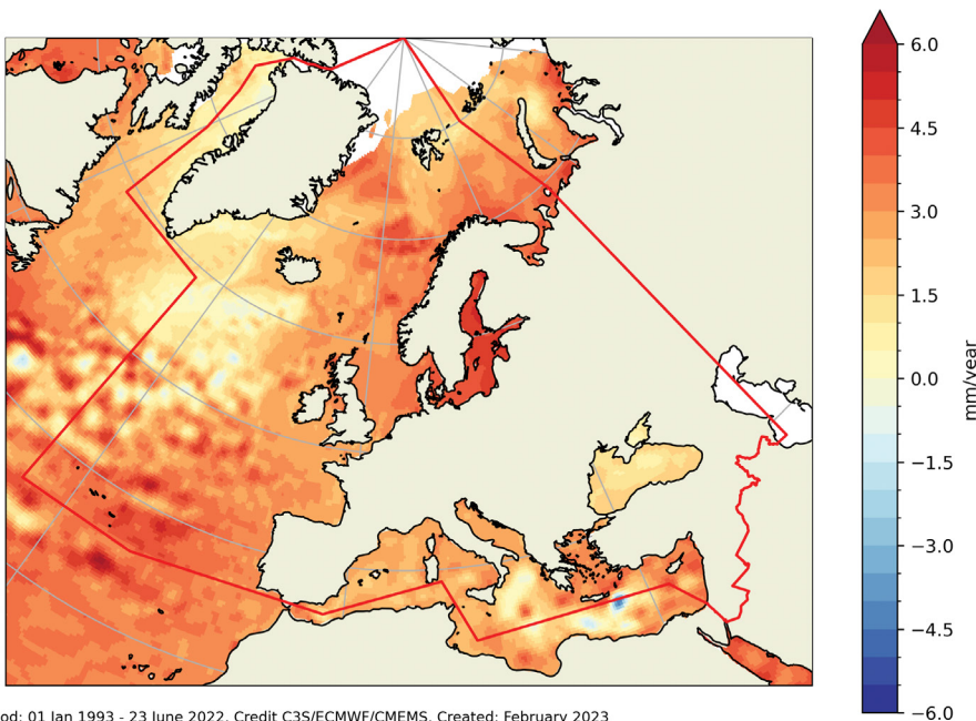
Figure 8. Sea-level trends (mm/year) from satellite altimetry from January 1993 to June 2022. The data have not been adjusted for glacial isostatic adjustment nor for the TOPEX-A instrumental drift. The red line indicates the WMO Region VI – Europe.
