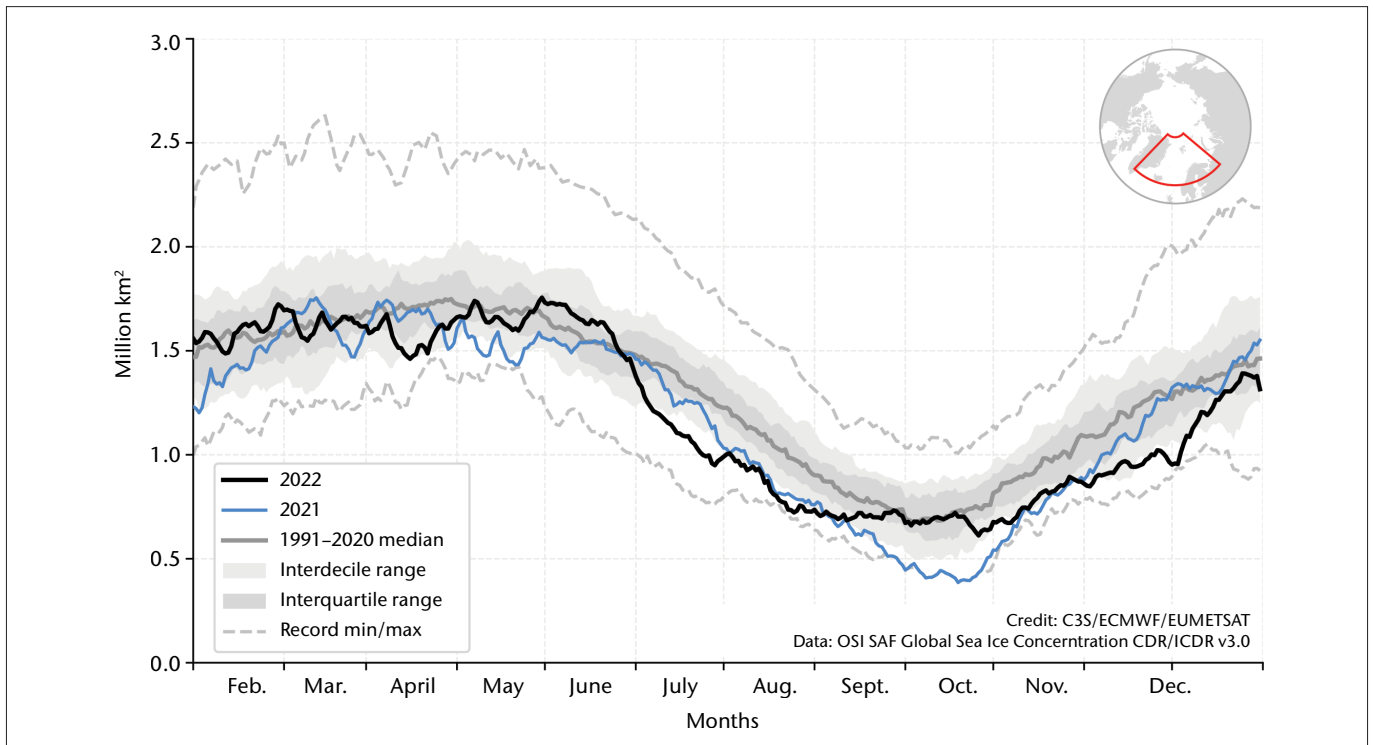
Figure 5. Total daily sea-ice extent in the European Arctic sector for 2021 (blue) and 2022 (black). The plot shows in grey shades the daily median (solid line), interdecile range (light shading) and interquartile range (dark shading) during the 1991–2020 reference period, as well as the daily minimum and maximum during 1979–2022 (dashed lines). The European Arctic sector is outlined in red on the inset map. Source: Sea-ice extent derived from the EUMETSAT Ocean and Sea Ice Satellite Application Facilities (OSI SAF) Global Sea Ice Concentration (Interim) Climate Data Record v3.0: https://osi-saf.eumetsat.int/products/osi-430-a
