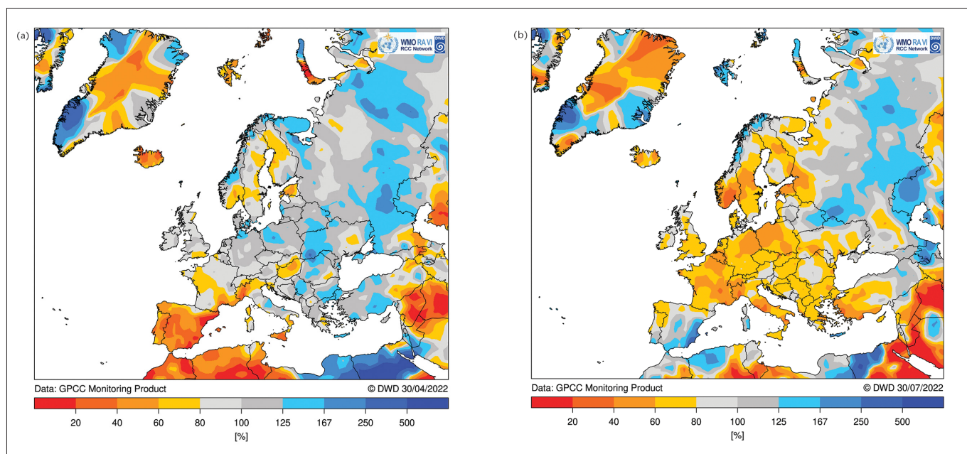
Figure 11. (a) Precipitation (percentage of the 1991–2020 average) for winter 2021/22 and (b) spring 2022 Source: Global Precipitation Climatology Centre (GPCC), DWD, Germany
