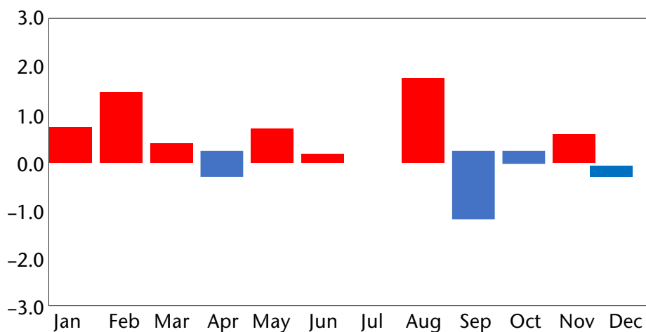
Figure 9. North Atlantic Oscillation (NAO) index monthly mean values, in 2022 Source: Data from the National Oceanic and Atmospheric Administration (NOAA) Climate Prediction Center (CPC)
