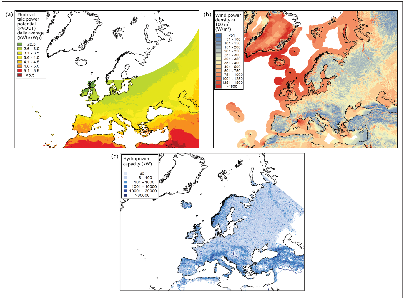
Figure 15. (a) Long-term average daily sum of electricity production from a 1 kW peak grid-connected solar PV power plant for the period 1994–2018; (b) An estimate of mean wind power density at 100 m above surface level globally for the period 1998–2017; (c) An estimate of potential hydropower (hydropower capacity)
