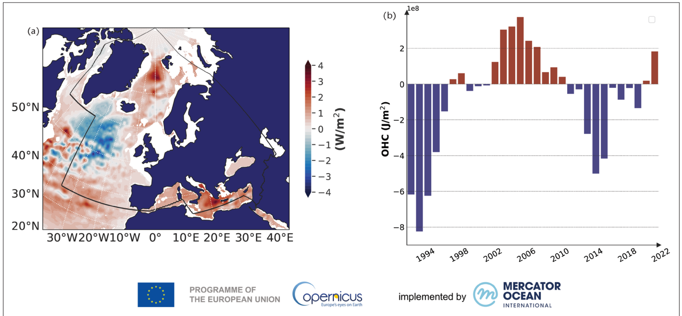
Figure 7. (a) Regional ocean heat content (0–700 m depth) anomalies for 2022 (relative to 2005–2022 climatology). The WMO area for Europe is indicated with a black line. White areas indicate regions where the ocean is shallower than 300 m, which have been excluded in this analysis due to limitations in ocean measurement density. (b) Ocean heat content annual anomalies over the period 1993–2022 (relative to 2005–2022 climatology). Source: Copernicus Marine Service/Mercator Ocean International, France, from an observational-based product distributed by the Copernicus Marine Service ( https://doi.org/10.48670/moi-00052 )
