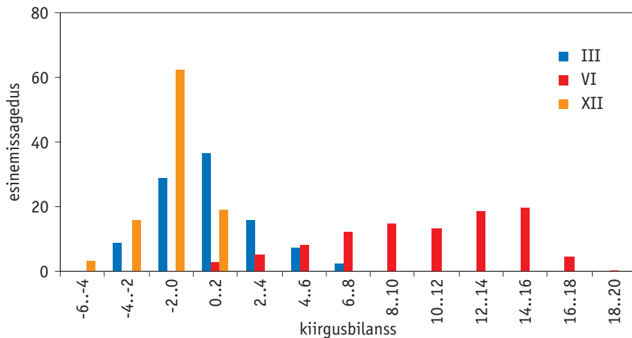
Fig. 10.6-9. Frequency of diurnal values of net radiation at Tõraveri in 1962-2000 (%).
