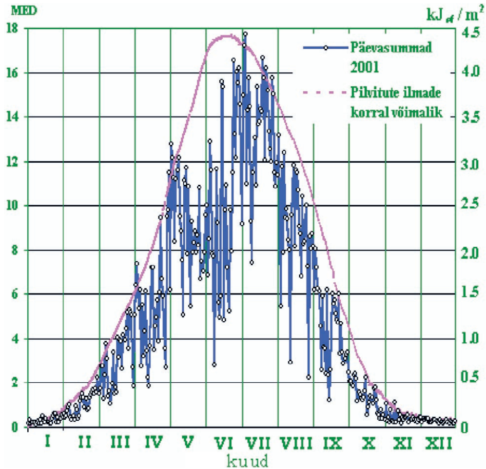
Fig. 10.5.3-4. Daily erythema UV-doses in 2001.
