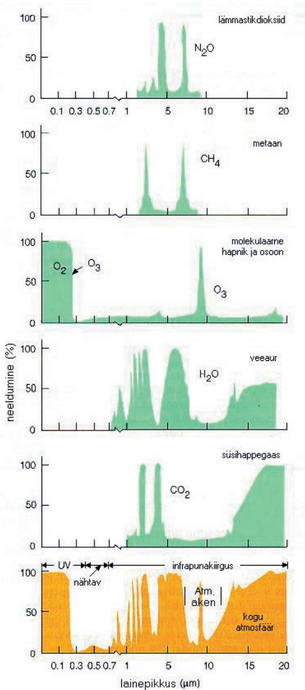
Fig. 4.1-4. Absorption of radiation by gases in the atmosphere (%).
