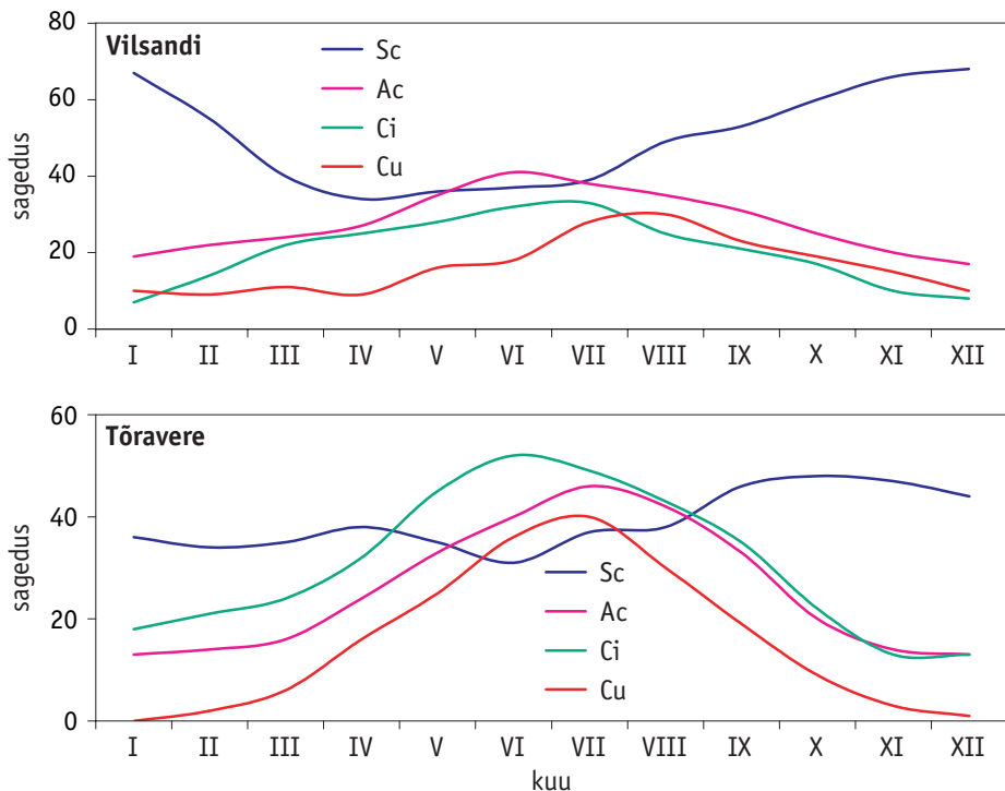
Fig. 7-8. Mean frequency of cloud genera as per cent from all observations at Vilsandi and Tõraveres (Spravochnik, 1968; Russak, 1990).
