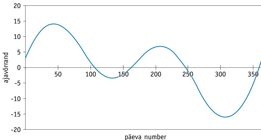
Fig. 3-2 Annual course of the equation of time.
