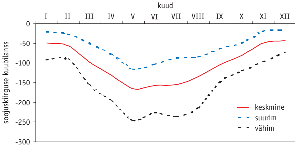
Fig.10.6-5. Annual course of mean and extreme monthly values of net long-wave radiation ( B_L ) at Tõravere in the period 1962-2000 ( \text{MJm}^{-2} ).
